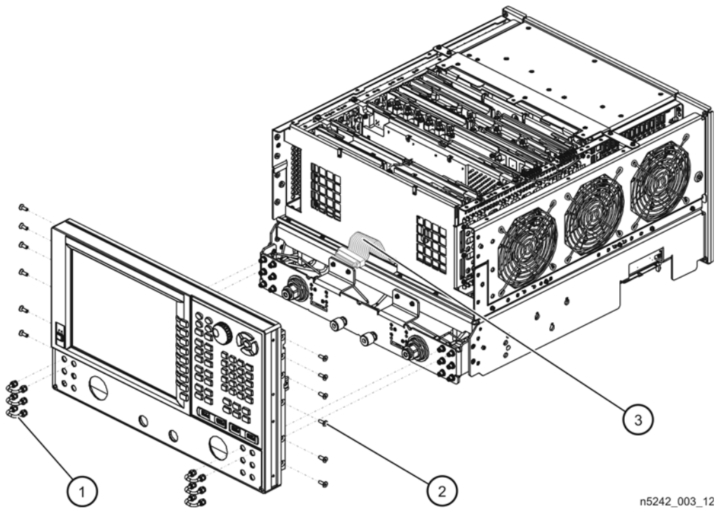
Figure 19 Front Panel Assembly Reinstallation
