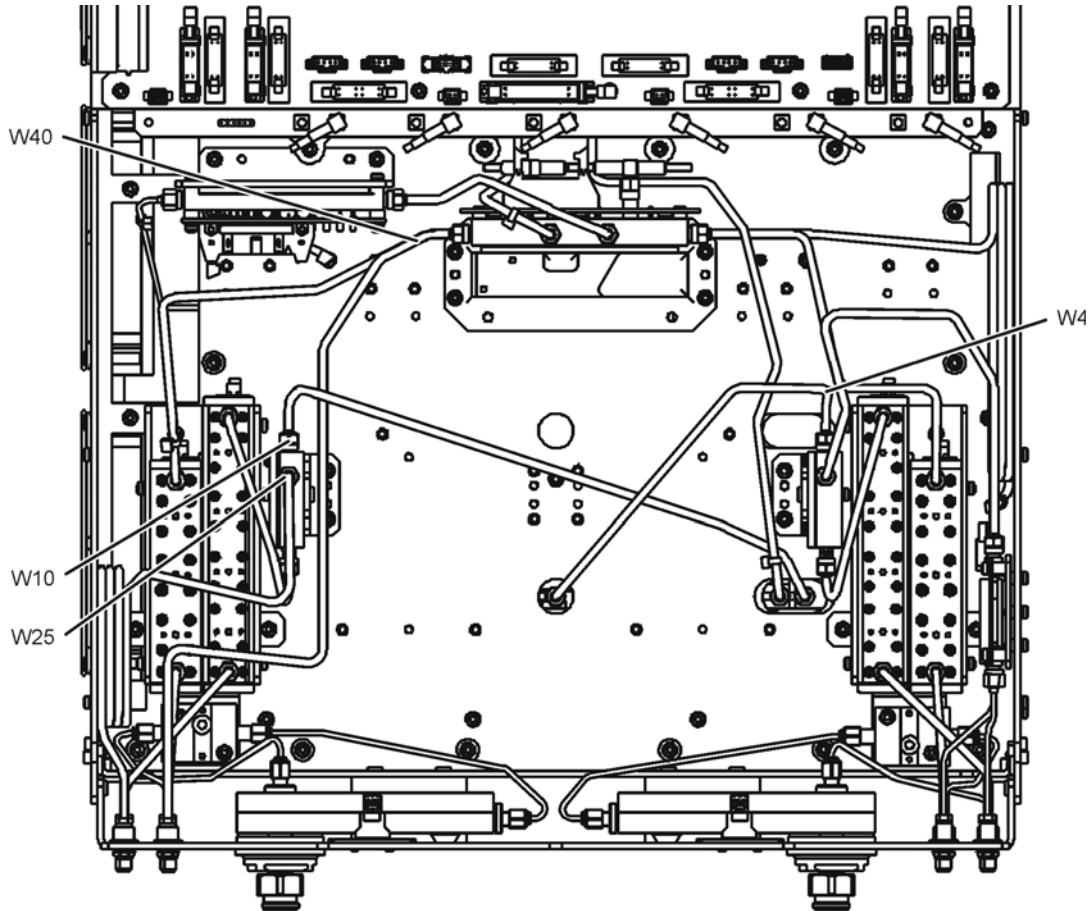
Figure 4 Existing Test Set Cables Removal
